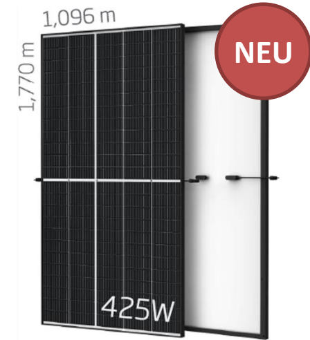
Vertex S+ TSM-NEG9.28
